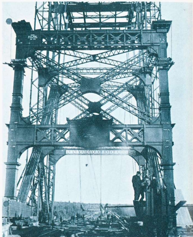
QUEBEC BRIDGE, A HISTORY OF DISASTER — The now famous bridge was started in 1900, collapsed on August 29, 1907 killing seventy-five workmen. Reconstructed in 1913, the bridge collapsed again on September 11, 1916 killing 13 more people. The bridge was finally constructed in 1917 and has remained standing since. The bridge was constructed to link Quebec City with the trade and commerce of the south shore on the St. Lawrence.
