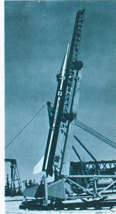
BLACK BRANT ROCKETS launched from the rocket range at Churchill, Manitoba measure the characteristics of the upper atmosphere.
